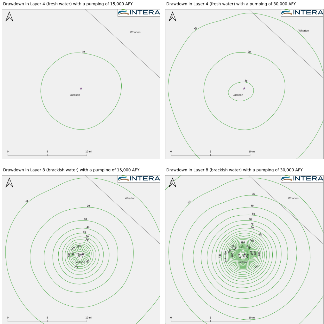
Figure 4-56. Simulated drawdowns after 5-year pumping at well field #1 at a rate of 15,000 AFY (left) and 30,000 AFY (right).
